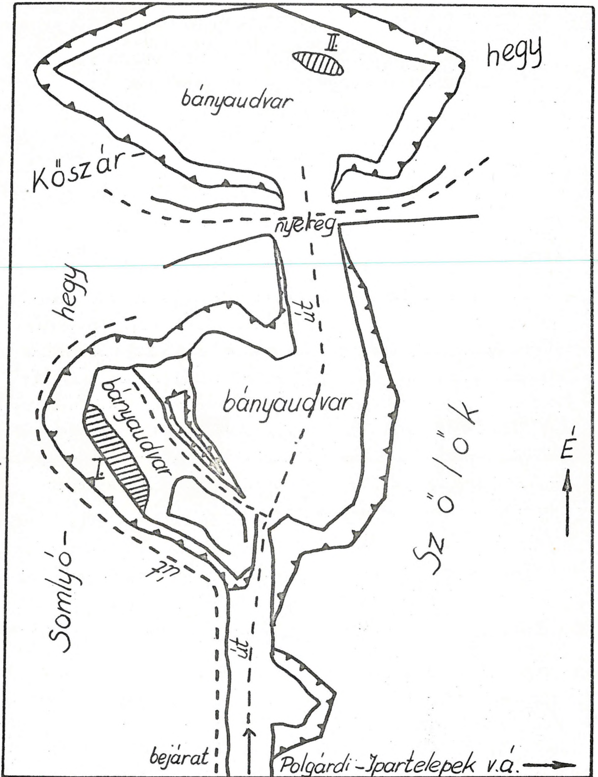
Fig. 1. Topographic outline of the big quarry at Polgárdi-Ipartelepek (I = Locality of KORMOS T.; II = The locality of the new occurrence of the Pikermi-type fauna)
