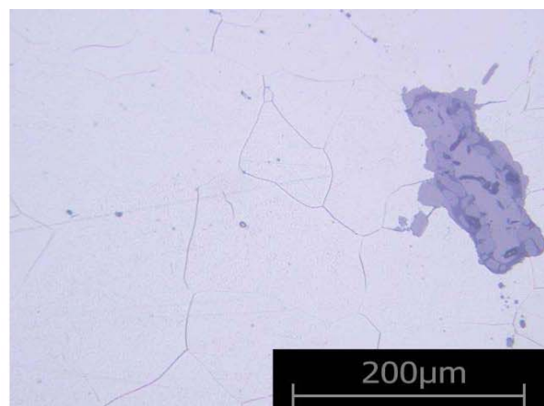
Fig. 4.: Metallographic picture of the bit-ring. On the left: micro hardness values. On the right: slag inclusion.
